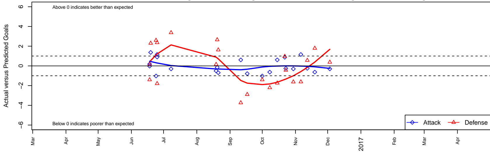
NW United Red G04 Dots are actual minus expected GF (blue circles) and GA (red triangles). Blue line is smoothed change in attack strength. Red is smoothed change in defense strength.
